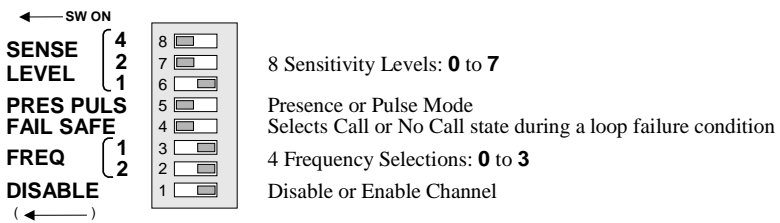
Front Panel Eight-position DIP Switch Module (Factory Default Settings Shown)
