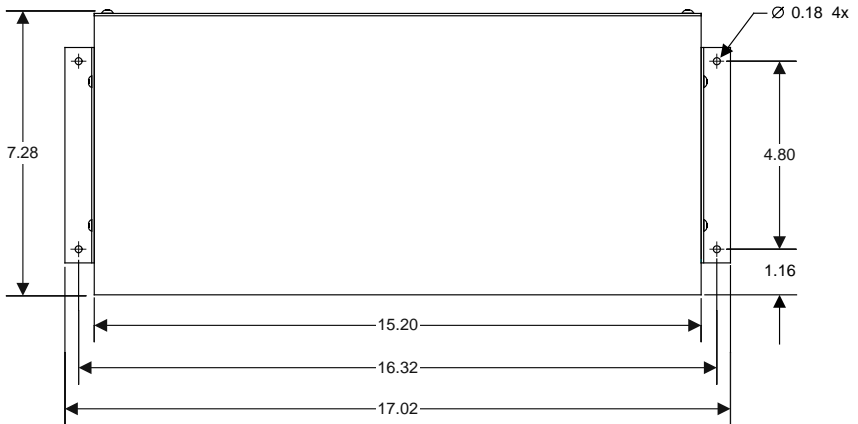
TOP VIEW - CARD RACK HEIGHT IS 6.27 INCH
